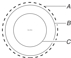
A. 1/2" (13 mm) maximum overhang B. Outer edge of cooktop C. Minimum pan size, if applicable
